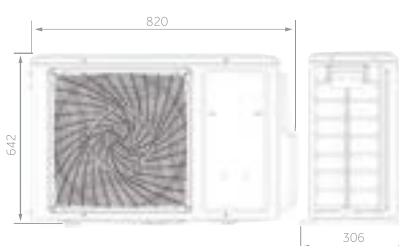
MOUNTING DIMENSIONS
