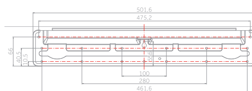
MOUNTING DIMENSIONS
